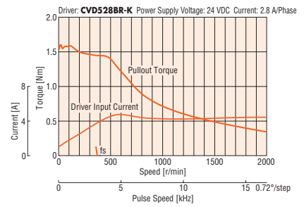
PKP568N28A2/PKP568N28B2
