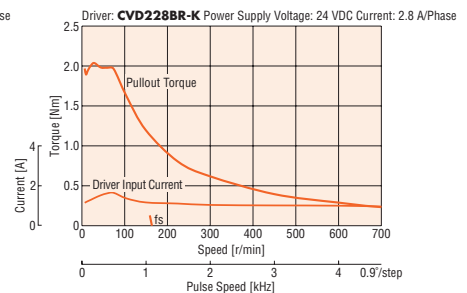
PKP268MD28A/PKP268MD28B
