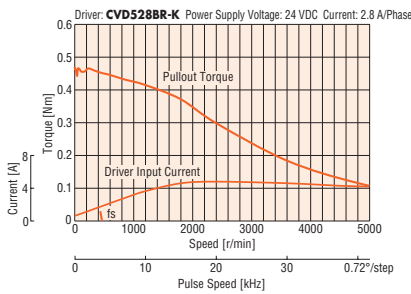
PKP564N28A2/PKP564N28B2
