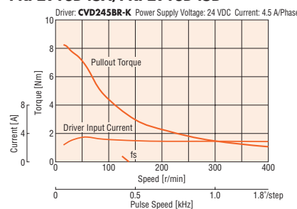
PKP2913D56A/ PKP2913D56B
