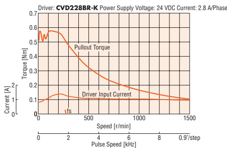
PKP264MD28A/PKP264MD28B
