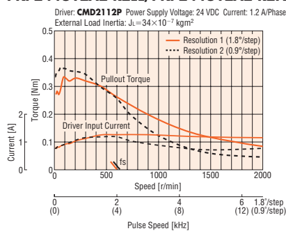
PKP244U12A2-R2EL/PKP244U12A2-R2FL
