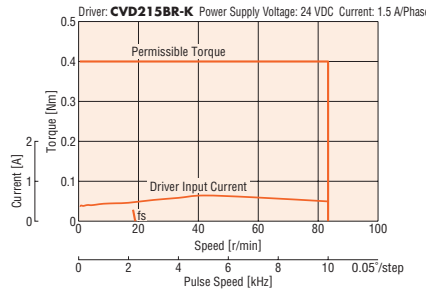
PKP223D15A-SG36/PKP223D15B-SG36
